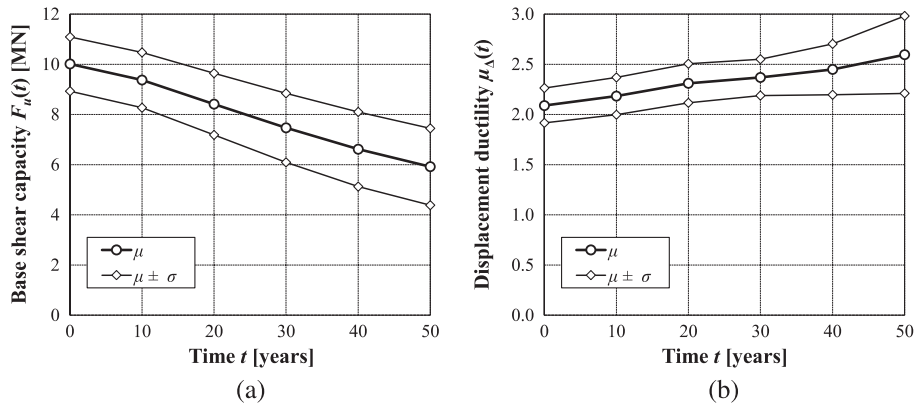
Figure 16. Bridge under corrosion. Time evolution of mean \mu and standard deviation \sigma of (a) base shear capacity F_u = F_u(t) and (b) displacement ductility \mu_\Delta = \mu_\Delta(t) .
