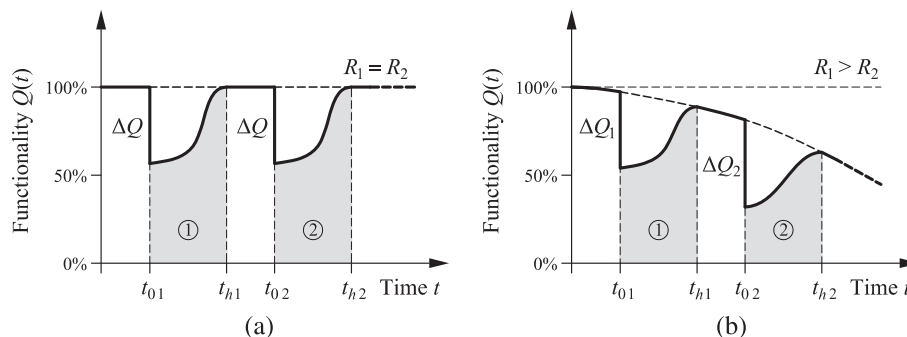
Figure 2. Functionality Q and functionality losses \Delta Q_k due to the occurrence of extreme events k = 1, 2, \dots , of same magnitude at different time instants t_{0,k} and recovery over the time intervals [t_{i,k}; t_{f,k}] , with t_{i,k} = t_{0,k} and t_{f,k} = t_{h,k} . (a) Non-deteriorating system and (b) deteriorating system.
