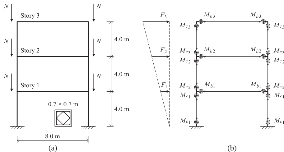
Figure 7. Three-story concrete-frame building. (a) Geometrical dimensions and column cross-section. (b) Structural modeling.
