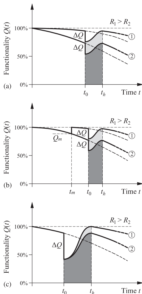
Figure 3. Effects of the deterioration process and related factors on the time-variant system functionality Q = Q(t) and resilience R = R(t_0) . (a) Environmental aggressiveness with ① slight/moderate exposure or ② severe exposure. (b) Maintenance programs ① with and ② without repair interventions. (c) Post-event recovery actions with ① total restoring of the initial functionality or ② partial restoring of the pre-event functionality.
