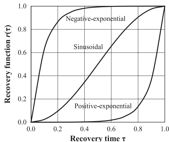
Figure 6. Functionality recovery profiles ( k=10 ).
