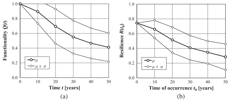
Figure 11. Frame building under corrosion. Time evolution of mean \mu and standard deviation \sigma of (a) system functionality Q = Q(t) and (b) seismic resilience R = R(t_0) for the case of t_i = t_0 , t_h = t_f , \delta_r = 12 months, functionality loss \Delta Q(t_0) = 0.5Q(t_0) , and recovery process with sinusoidal profile and partial restoring aimed at recovering the pre-event functionality.
